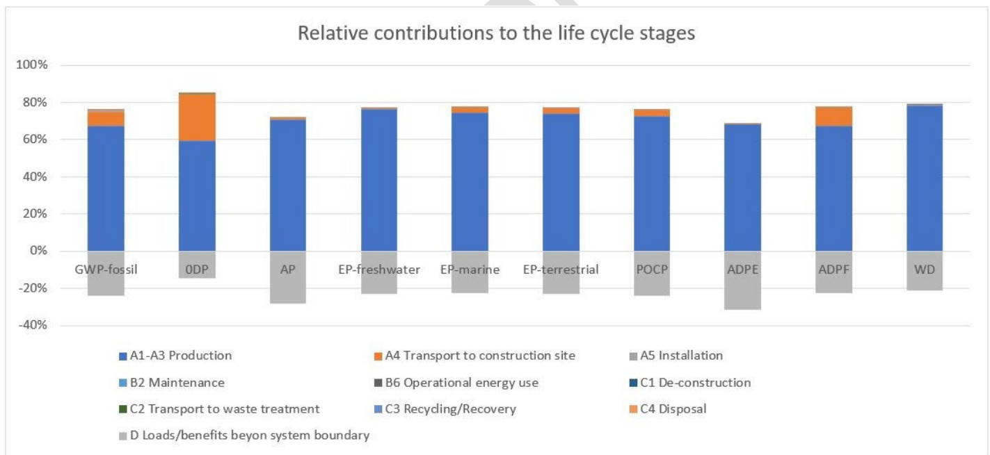
Figure 1: Environmental impacts of locks (L) along its life cycle (impacts from production modules A1-A3 = 100 %)
